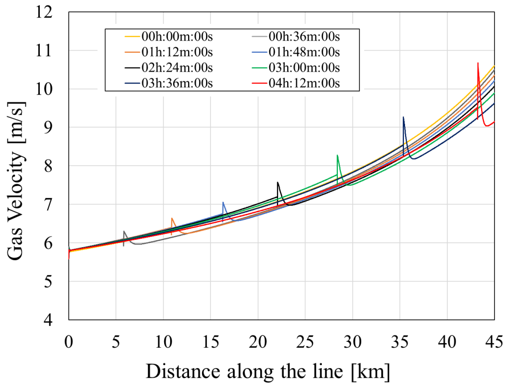
Figure 9.44: Gas velocity profile with ModFORCE method and 5E2P, two-phase pigging.
