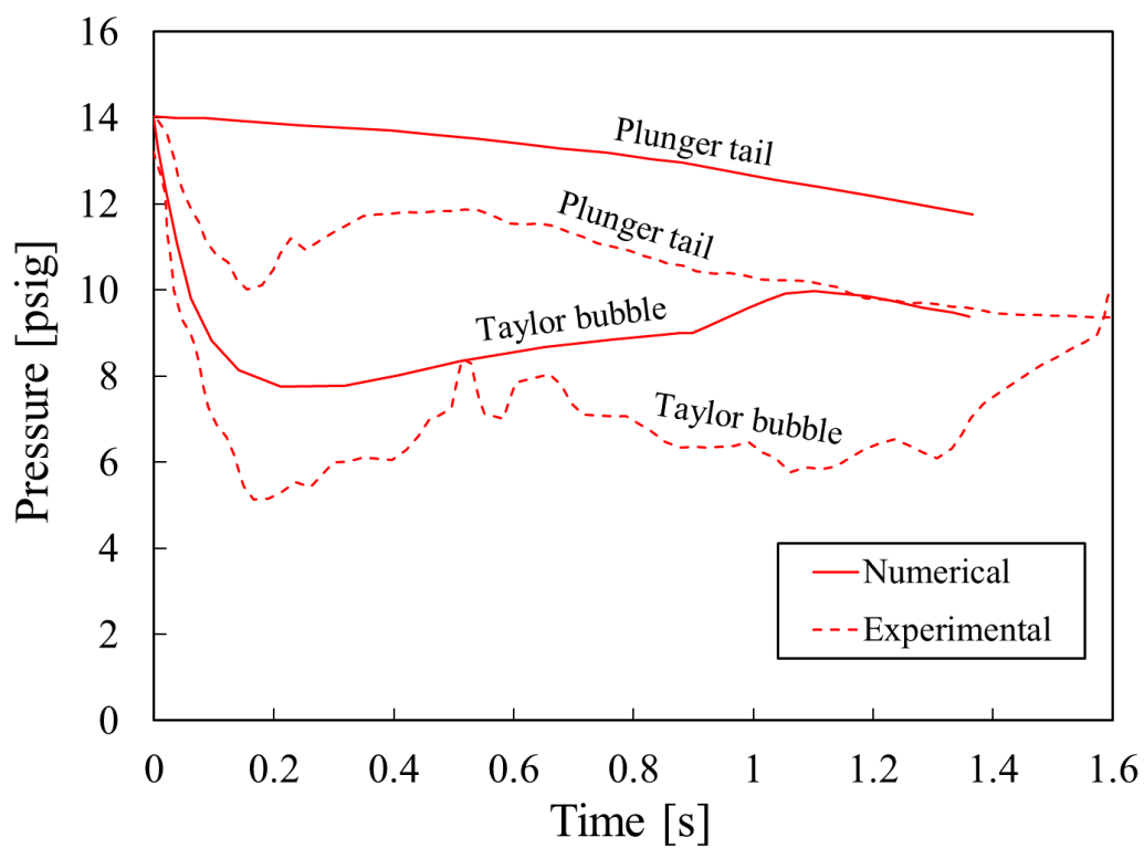
Figure 10.10: Pressure against time (14psig), logging plunger case.
