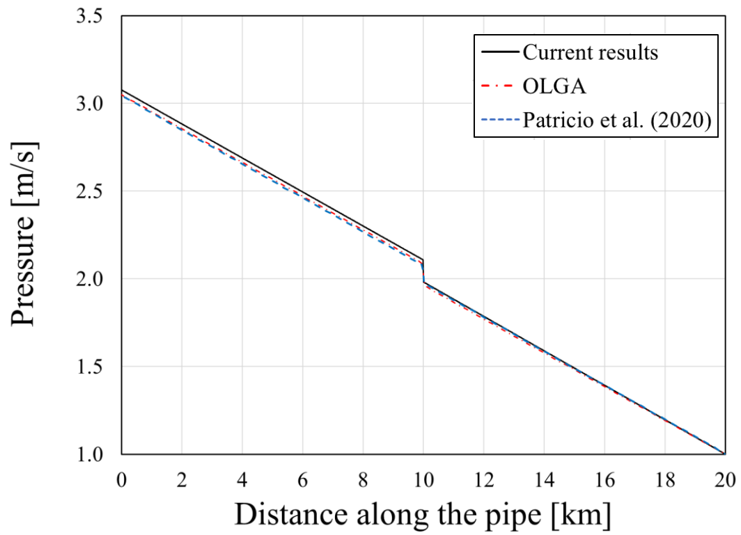
Figure 9.8: Pressure profile comparison for the pigging in liquid flow case.
