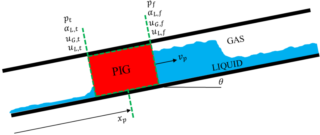
Figure 7.5: Sketch for a Two-phase flow bypass pig.
